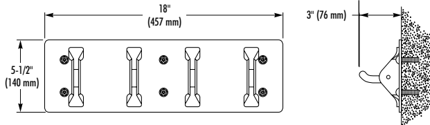
MODEL SA39
